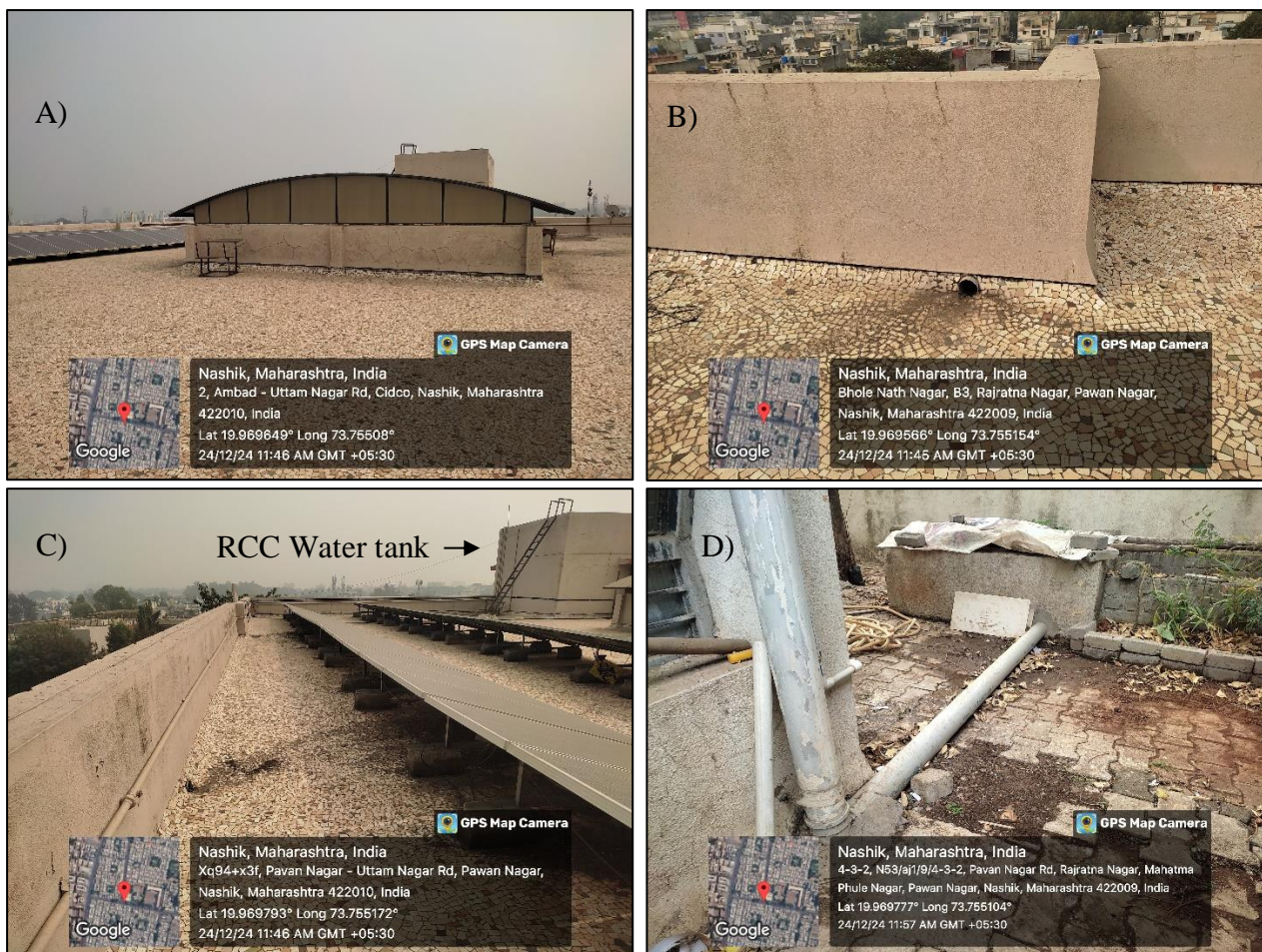
Figure A), B) & C) Terrace of the building with dome and water inlets to the water storage Figure D) Rainwater storage tank
